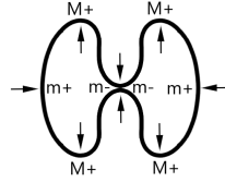
Figure 4 A single curve with a tangent point.
